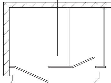
C569-XXNSIAH-XXXX Privacy, Left Latch Out & Left Hinge In / Right Hinge Out & Right Latch In
