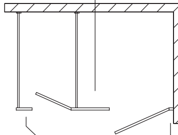
C569-XXNSIBH-XXXX Privacy, Right Hinge In & Right Latch Out / Left Latch In & Left Hinge Out
