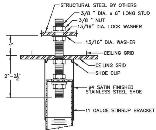
CEILING BOLT DETAIL
