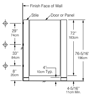
2090 Series Floor-Anchored
