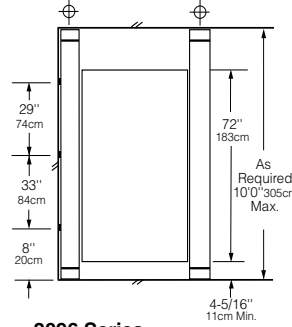
2096 Series Floor-to-Ceiling Anchored
