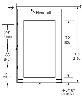
2092 Series Overhead-Braced
