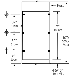
2093 Series Post-to-Ceiling Screen
