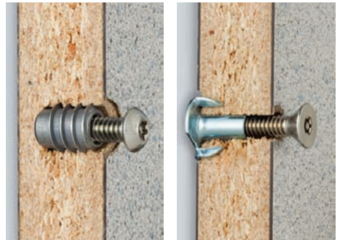
THREADED INSERTS, T-NUTS Factory installed. Provide metal-to-metal contact for securing door hinges and latch track.
