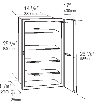
B-398 Unit combines adjustable shelves, mirror, used razor blade slot, and toothbrush holder.
